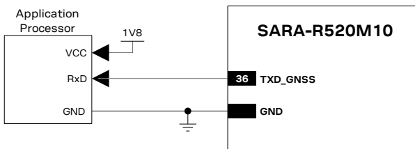
Figure 65: Application circuit for GNSS peripheral UART data output pin
