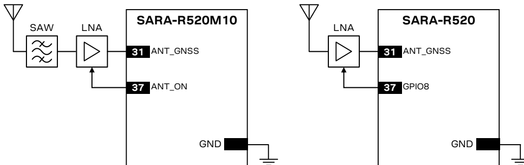
Figure 38: Example for best performance and improved jamming immunity with GNSS passive antenna placed far away
