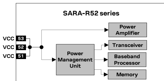
Figure 5: SARA-R52 series modules’ internal VCC supply routing
