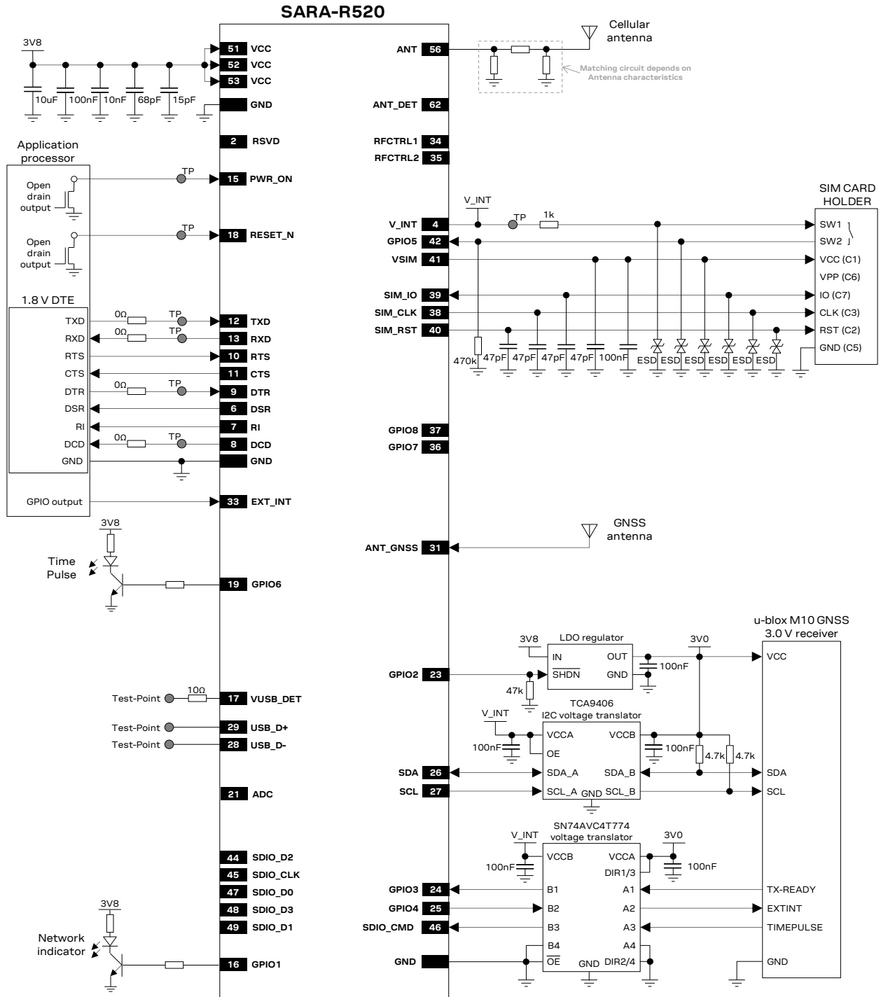
Figure 69: Example schematic diagram integrating a SARA-R520 module
