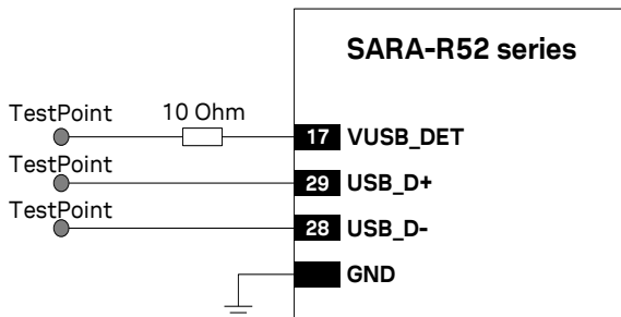
Figure 61: SARA-R52 series modules USB application circuit providing access for diagnostic purposes
