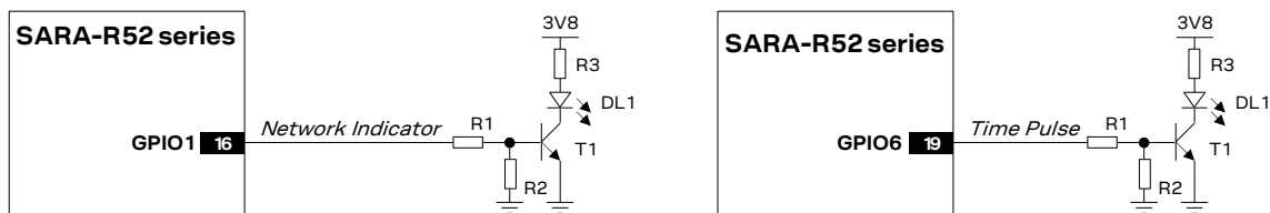
Figure 64: Application circuit for network indication provided over GPIO1 and/or time pulse provided over GPIO6
