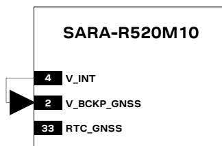
Figure 67: GNSS RTC application circuit with clock generated internally
