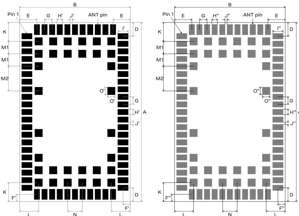
Figure 68: SARA-R52 series modules suggested footprint and paste mask (application board top view)
