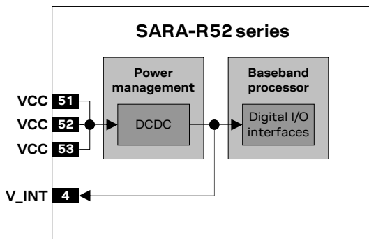
Figure 9: SARA-R52 series interfaces supply output (V_INT) simplified block diagram
