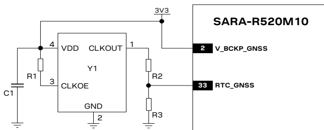
Figure 66: GNSS RTC application circuit with clock provided externally
