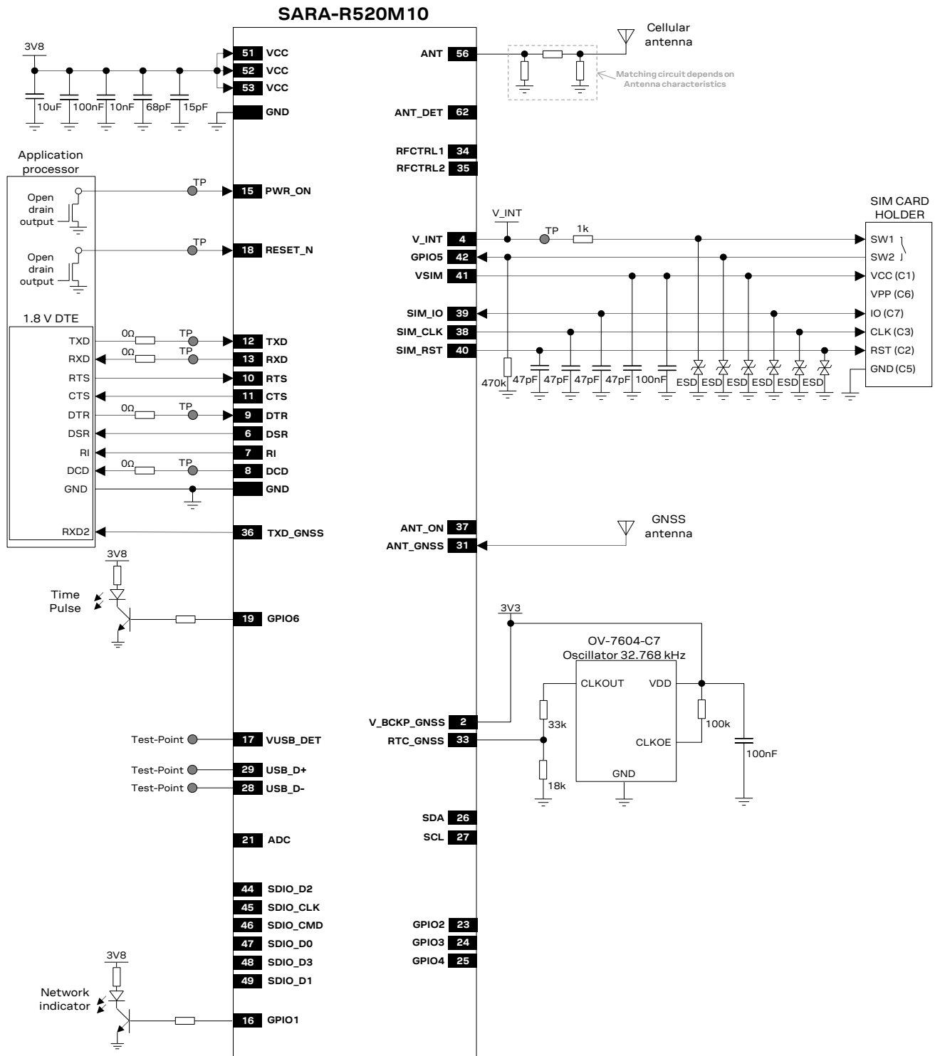
Figure 70: Example schematic diagram integrating a SARA-R520M10 module
