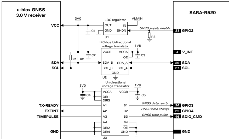
Figure 63: Application circuit for connecting SARA-R520 modules to a u-blox 3.0 V GNSS receiver
