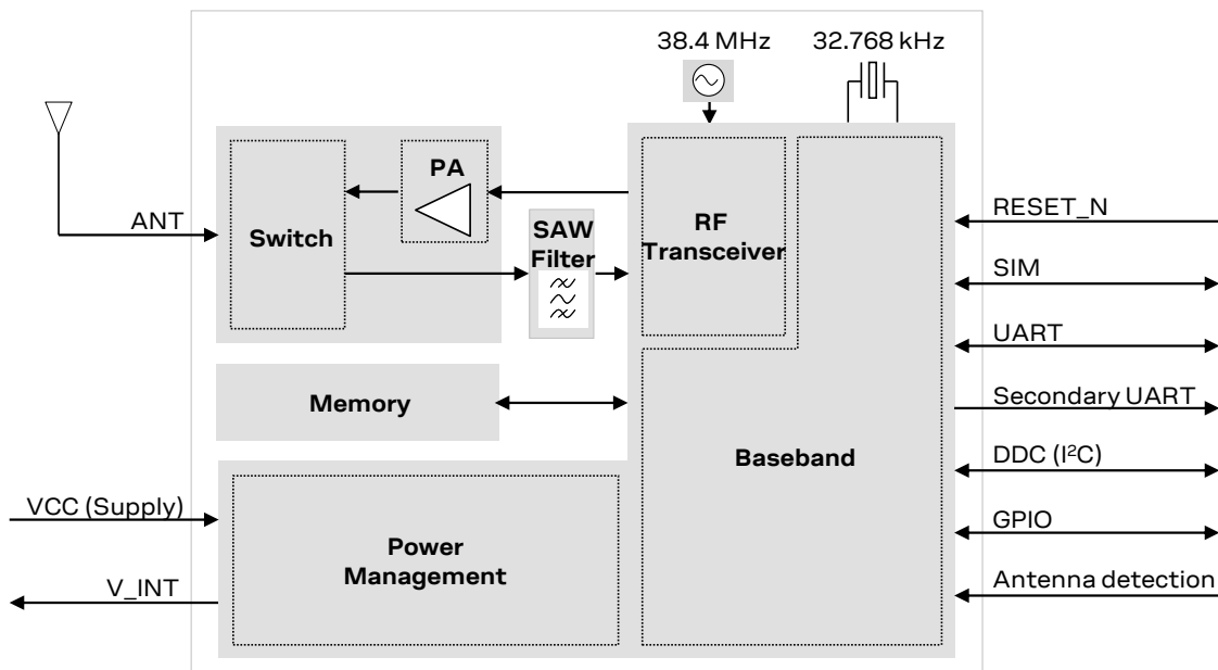
Figure 1: SARA-N2 series series block diagram
