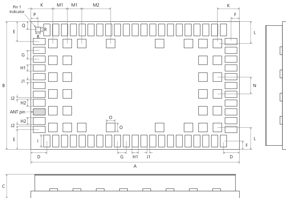
Figure 3: SARA-N2 series series dimensions (bottom and side views)
