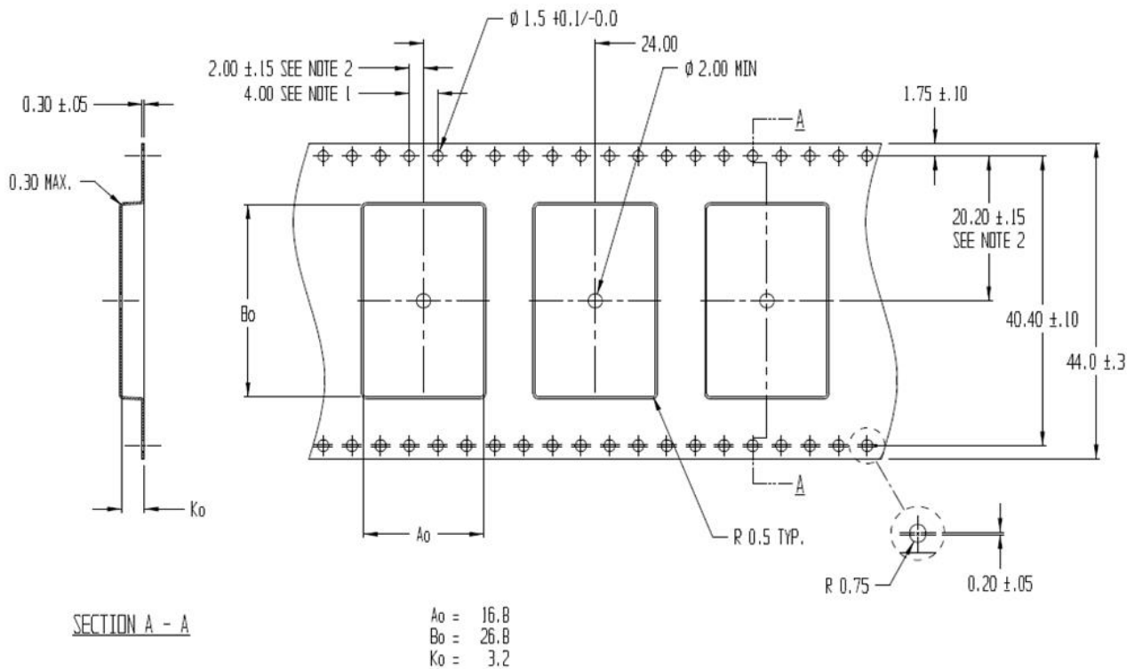
Figure 5: Dimensions for SARA-N2 series series on tape
