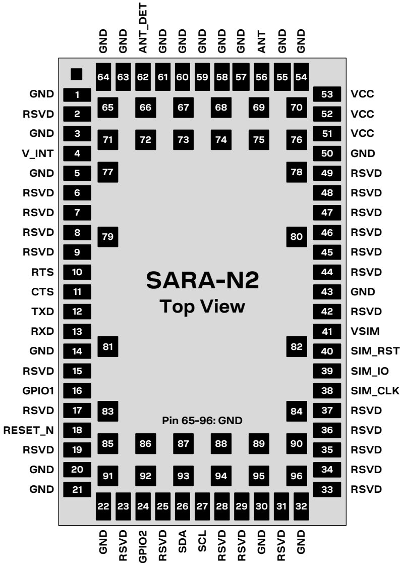
Figure 2: SARA-N2 series series modules pin assignment
