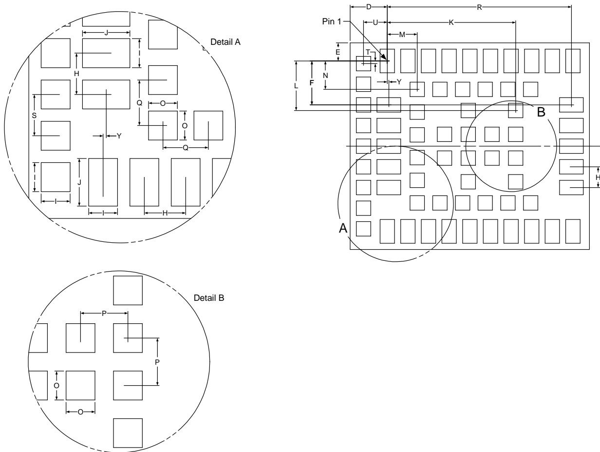
Figure 8: NINA-B41 pad dimensions
