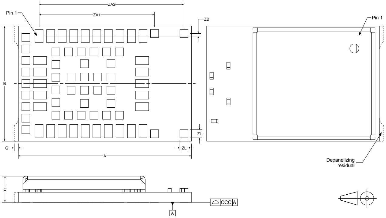
Figure 7: NINA-B416 mechanical outline data
