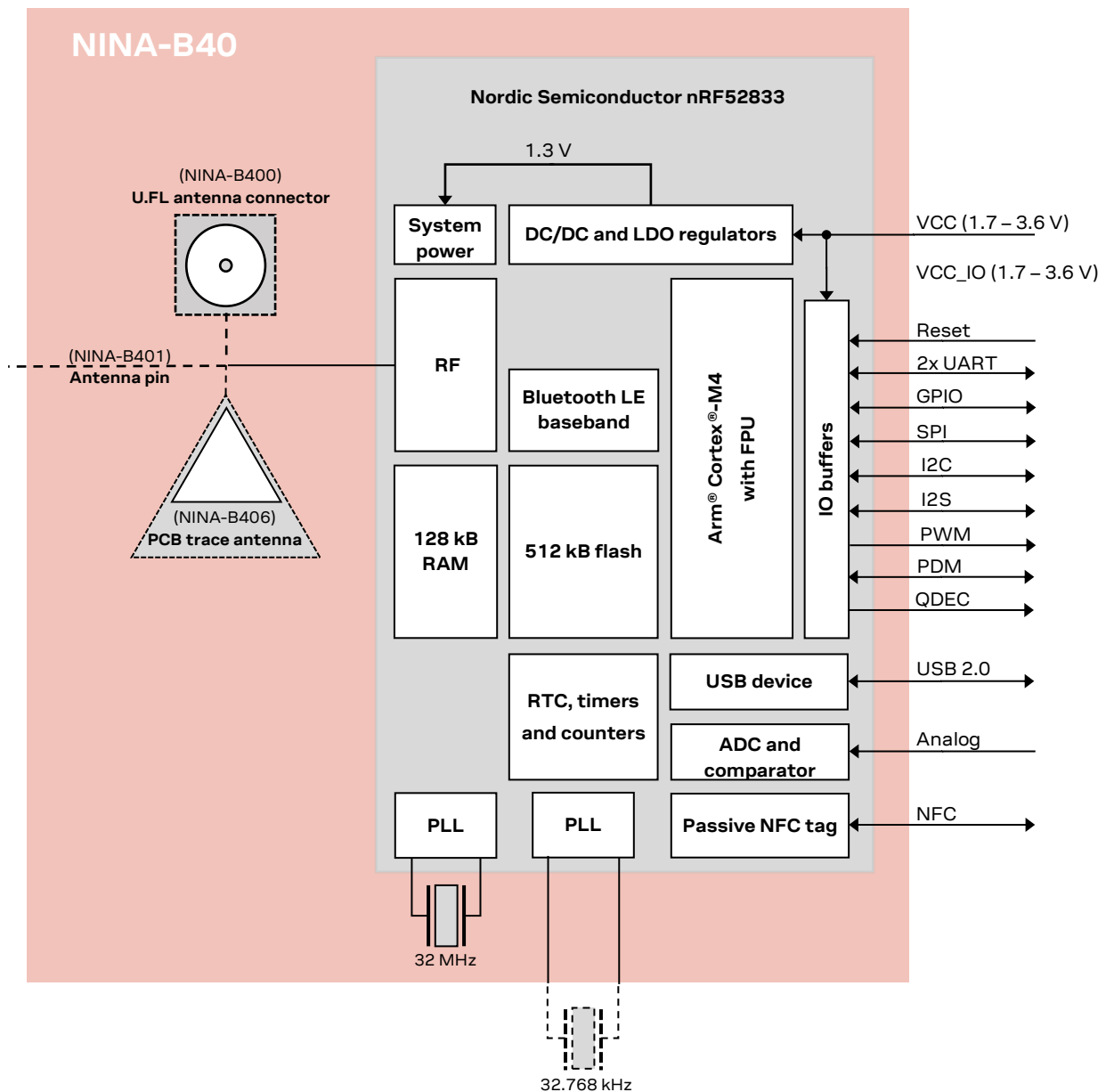
Figure 1: Block diagram of NINA-B40 series
