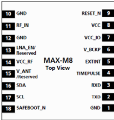
Figure 2: Pin Assignment
